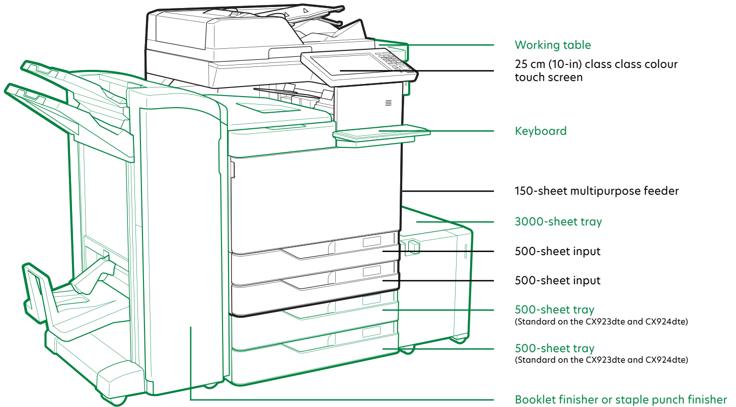
Staple finisher (not compatible with CX924)
